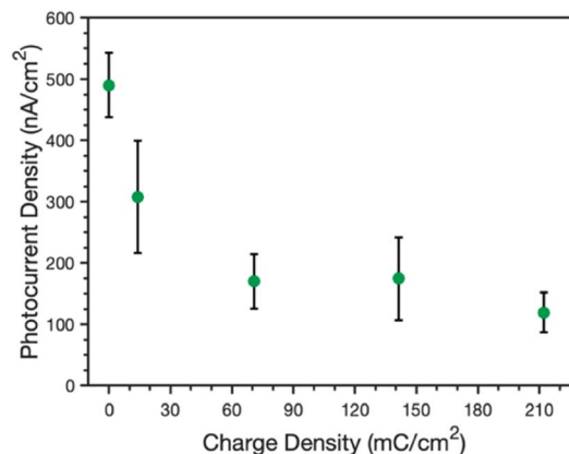
Fig. 7 Effect of charge density of electrodeposited PPy on the peak photocurrent density of PSI/Au films. Measurements were made in 0.1 M KCl (aq) containing AsC 2 H/DCPIP (20 : 1 mM) as redox mediators. All films were illuminated for 30 s and the peak current typically occurred within the first 2 s.
